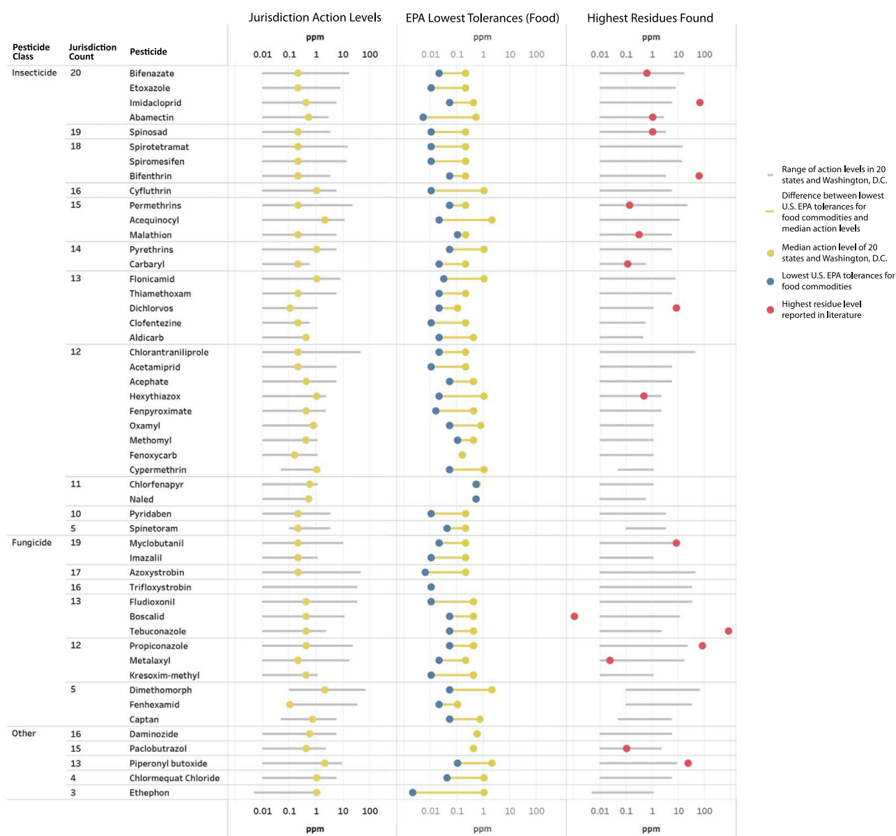
Fig. 3. Barbell plots of the top 50 pesticides with the largest variation of action levels in 20 states and Washington, D.C. The blue dots indicated the lowest U.S. EPA tolerances for food commodities, which are adopted for cannabis and cannabis-derived products in seven states. The red dots indicated the highest values of pesticide residues in cannabis plant matter as reported in the open literature (Supplemental Material S2). (For interpretation of the references to color in this figure legend, the reader is referred to the web version of this article.)
